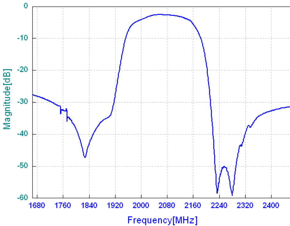
Frequency Response
